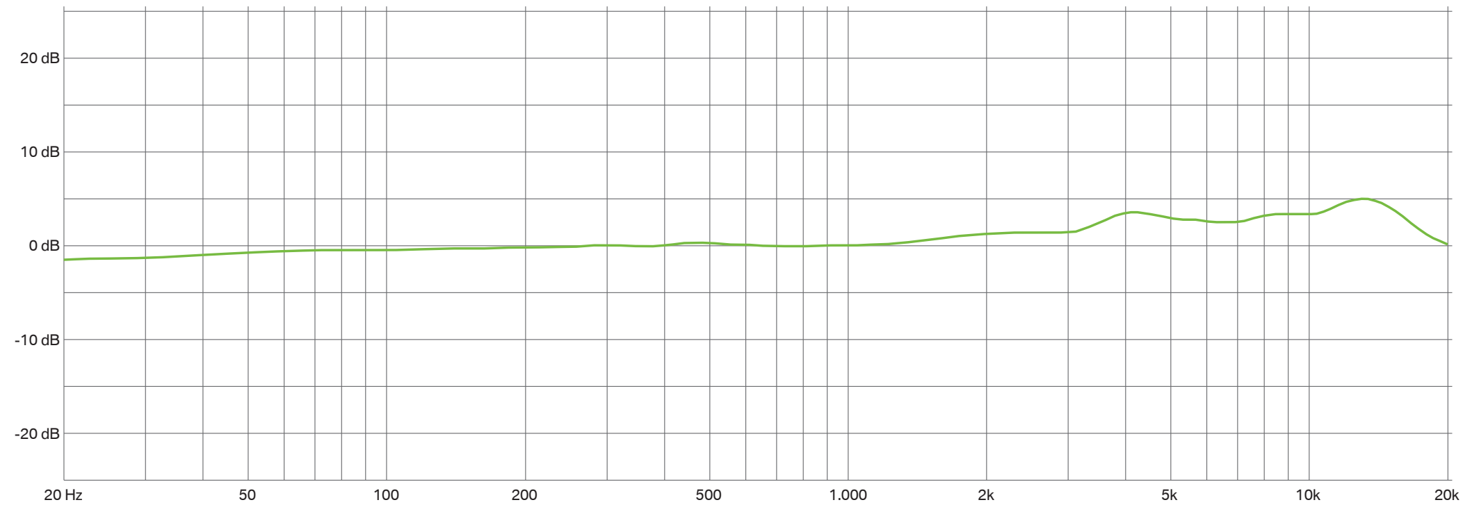
Figure 9.1 - Frequency response of the LCT 440 PURE
